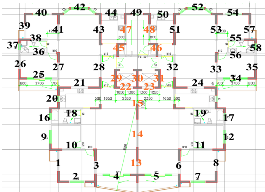
Fig. 9 Precast Walls Installation Plan
