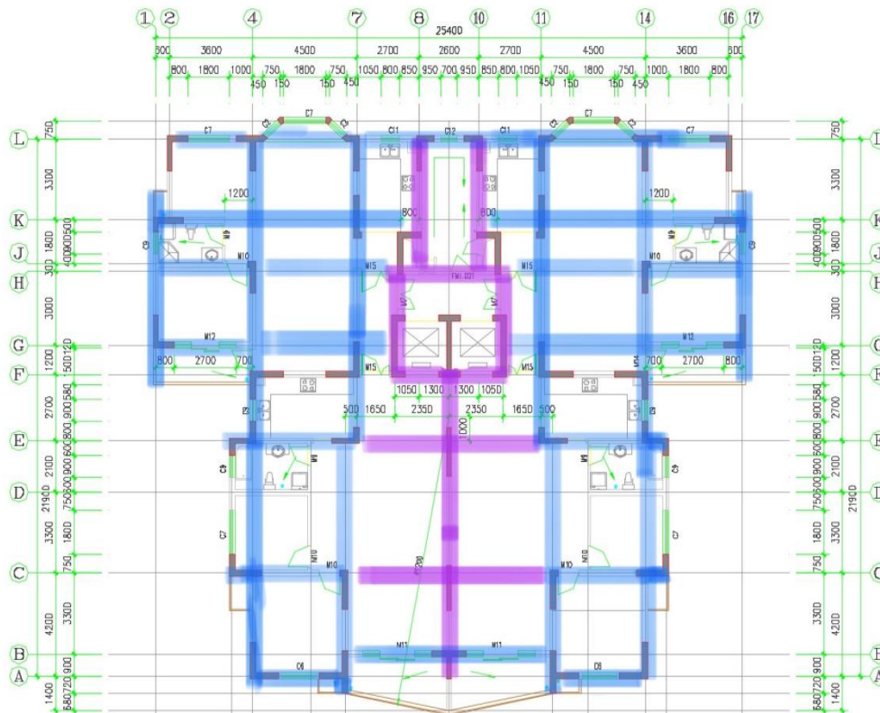
Fig 10. Arrangement of Precast Beams
