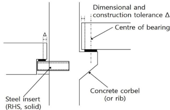
Fig. 3 Hong [7] details of pinned connection; beam resting on column corbel.
