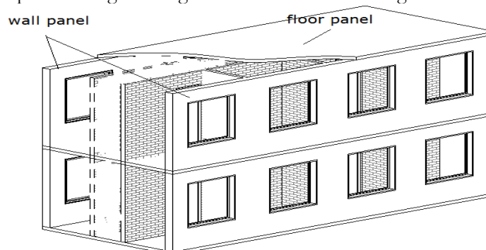
Fig.1 Long Wall Large Panel System, Redrawn from UNDP/UNIDO Project [2]
