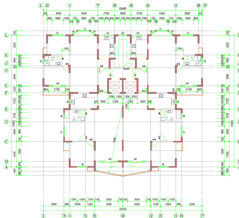
Fig 4. Floor plan for 8 story Residential Apartment
