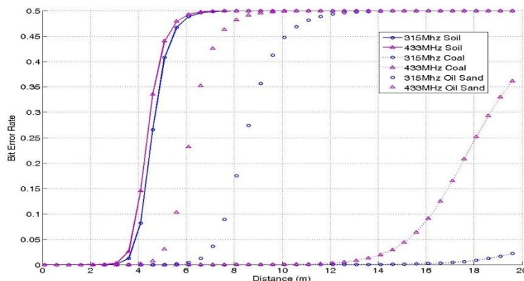
Fig. 3. BER for deep environment for 315/433 MHz a) for solids b) for liquids
