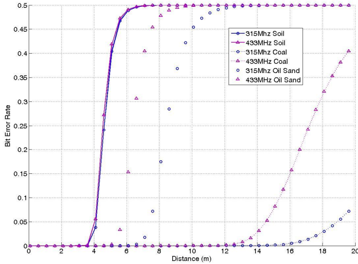
Fig.8. BER for shallow environment as a function of depth for 315/43 MHz a) for solids b)for liquids
