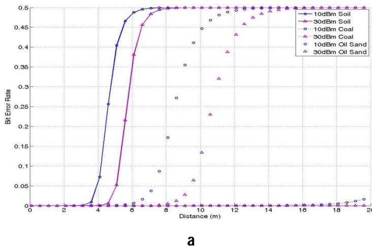
Fig. 4. BER for deep environment with transmission power 10-30 dBm at 315 MHz a) for solids b) for liquids
