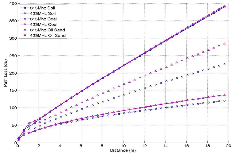
Fig. 6. Path loss for shallow environment for 315/43 MHz a) for solids b) for liquids
