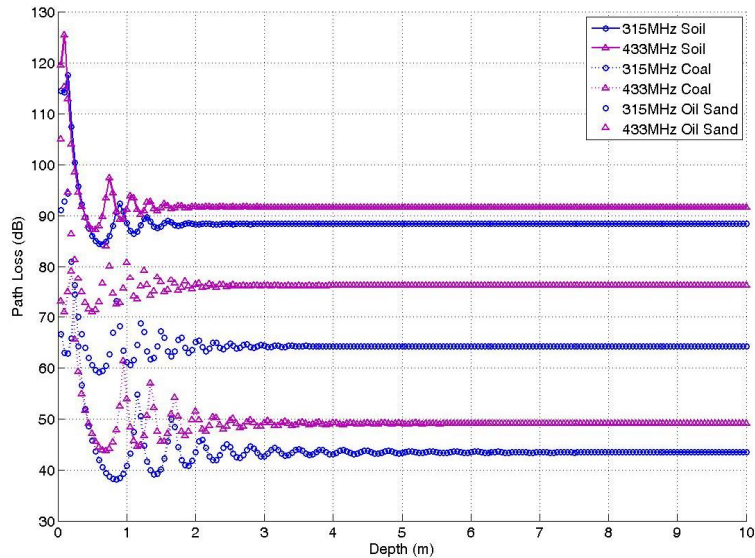
Fig. 7. Path loss for shallow environment as a function of depth for 315/43 MHz a) for solids b)for liquids
