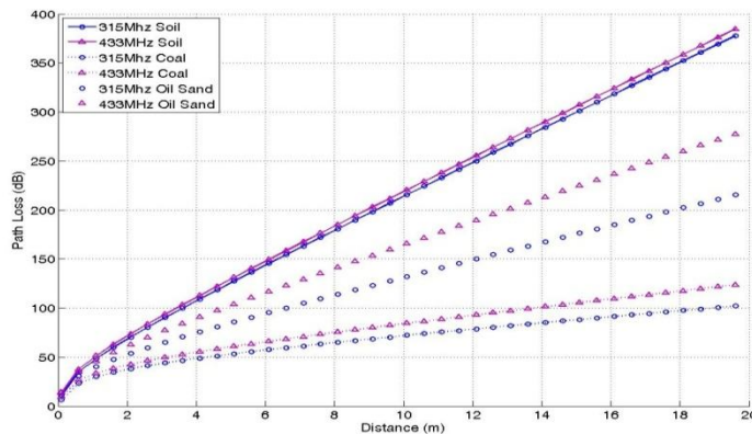
Fig. 2. Path loss for deep environment for 315/43 MHz a) for solids b) for liquids
